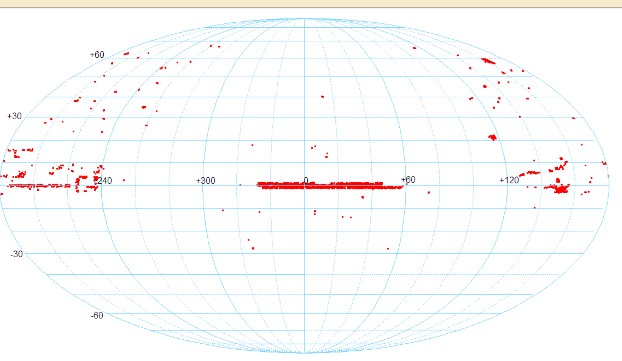
Figure 1 : The celestial distribution of the 1809 AGNs analyzed in this work. (equatorial coordinate)
