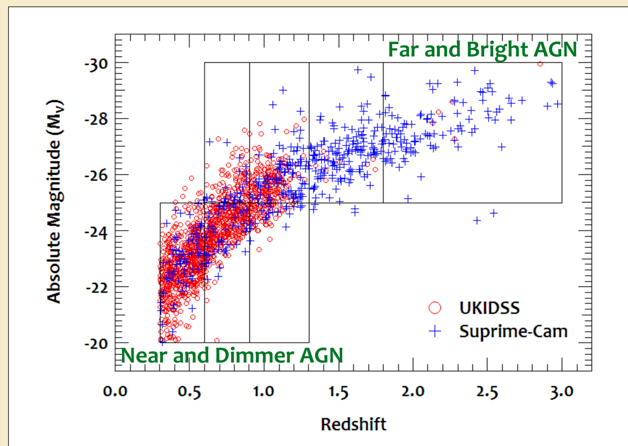
Figure 2 : K-corrected V band absolute magnitude vs redshift of the AGNs used in this work.
