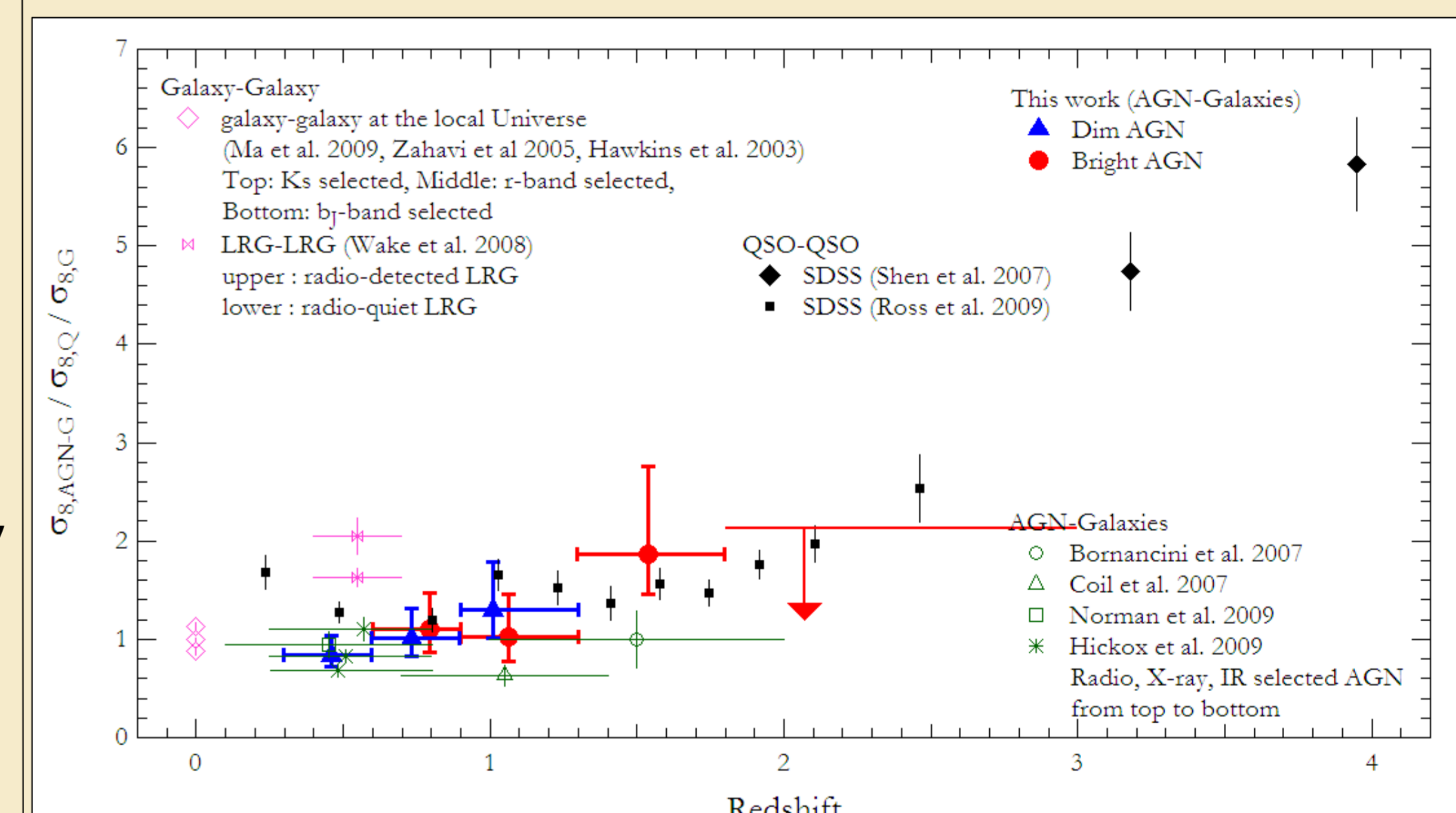
Figure 4 : The \sigma_8 of the galaxies around AGNs as a function of redshift.
